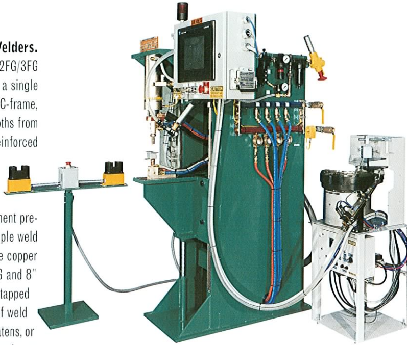
This C-Frame Welder is featured here with additional accessories.
