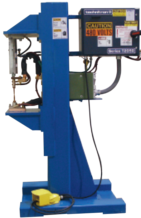
This C-Frame Welder is featured here with additional accessories.
